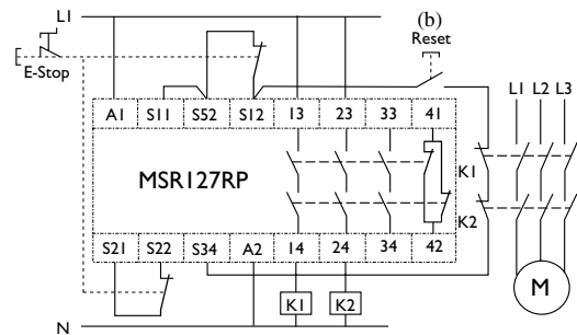
(c) Dual Channel E-Stop, Manual Reset, Monitored Output
