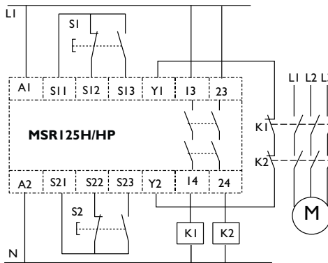
(b) Two-Hand Control, Dual Channel, Auto Reset, Output Monitoring
